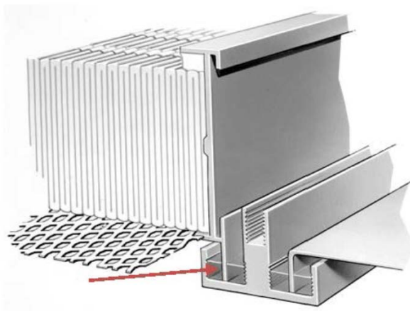
Figure ARG 3.B. Schematic showing how the “knife edge” of a HEPA filter is embedded into a silicone gel (red arrow) to form a leak-proof seal in a fan-HEPA filter unit.
