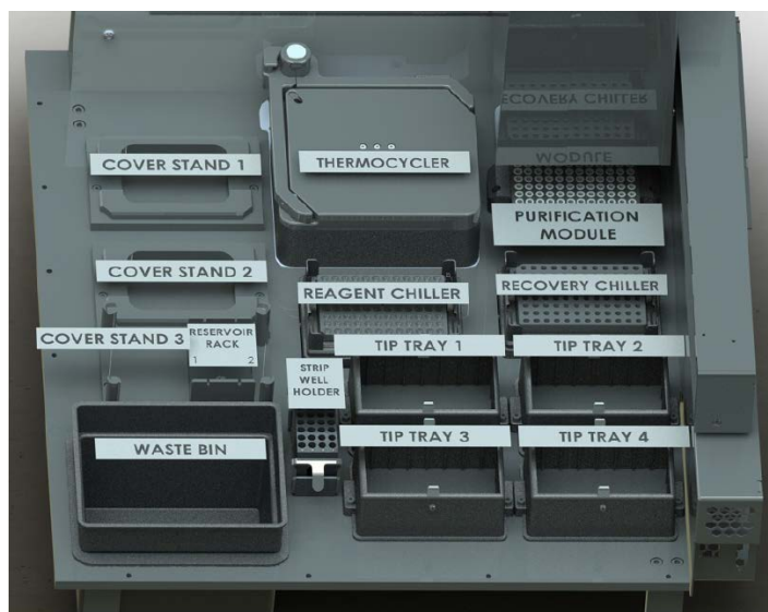
Figure 10.C. Different views of a DNA assembler. Exterior with the workspace area closed (top left), exterior with the workspace area open (top right), interior workspace with different areas labeled (bottom).
