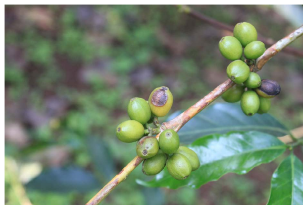
Figure PF1.A. Coffee bean plant with coffee berry disease infection.
