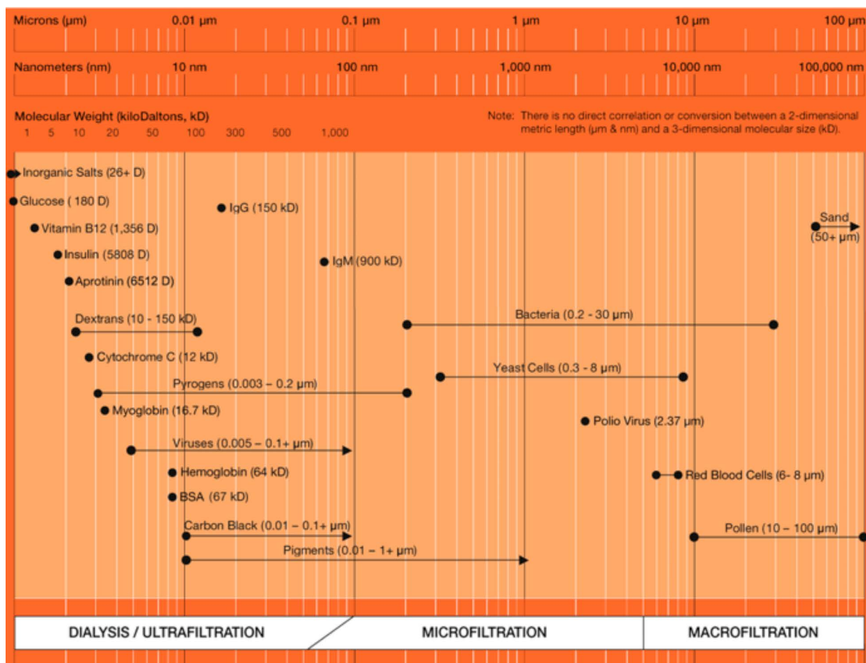
Figure 4.G. Filter pore sizes for different biological and chemical substances. 105
